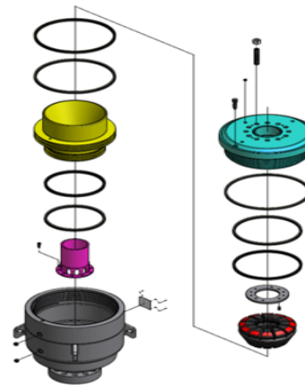
IK™ (GK Style) Annular BOP Seal & Component Parts Breakdown
