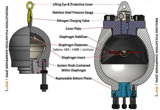
INTEGRATED DIAPHRAGMS IPD™ STYLE | IKD™ STYLE | EMSCO STYLE INTEGRATED PPD & DPD PULSATION DAMPENERS INTEGRATED PULSATION DAMPENERS (IPD™ | IKD™)
