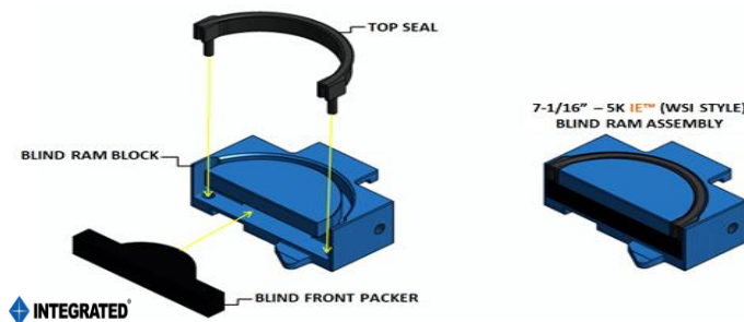
IE™ BLIND RAM ASSEMBLY
