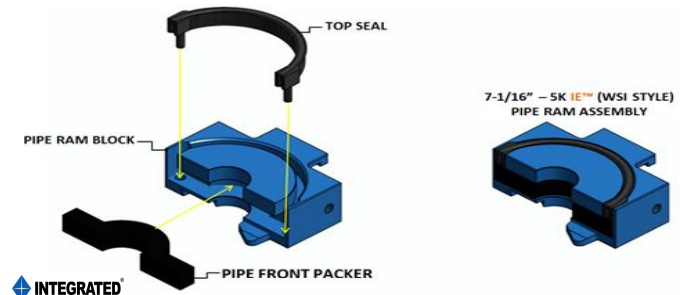
IE™ PIPE RAM ASSEMBLY
