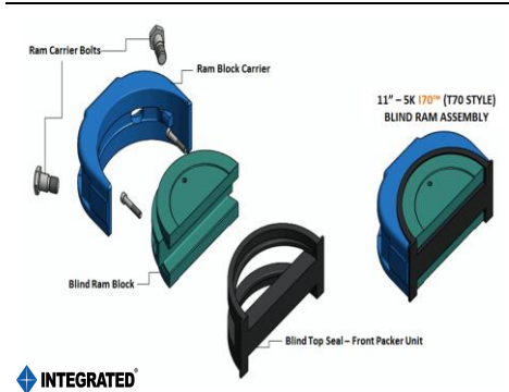
I70™ BLIND RAM ASSEMBLY
