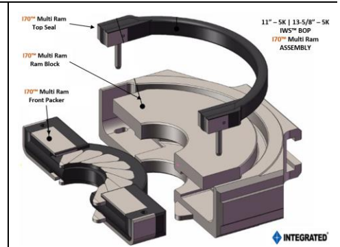
I70™ MULTI RAM ASSEMBLY
