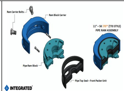
I70™ PIPE RAM ASSEMBLY
