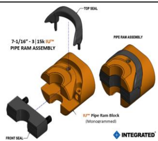
IU™ PIPE RAM ASSEMBLY
