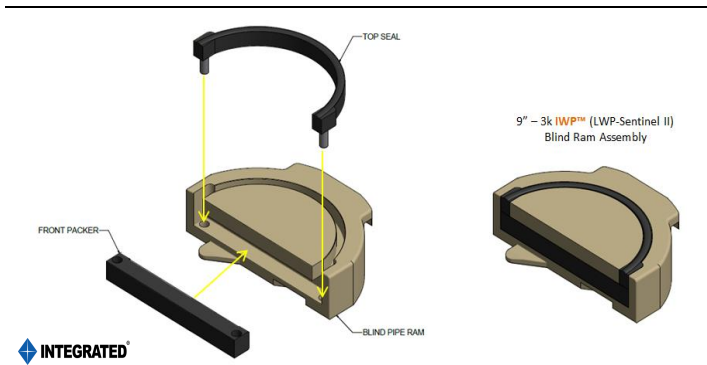
IWP™ BLIND RAM ASSEMBLY
