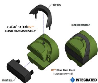
IU™ BLIND RAM ASSEMBLY
