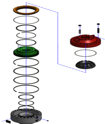
ISA™ (Spherical Style) Annular BOP Seal & Component Parts Breakdown
